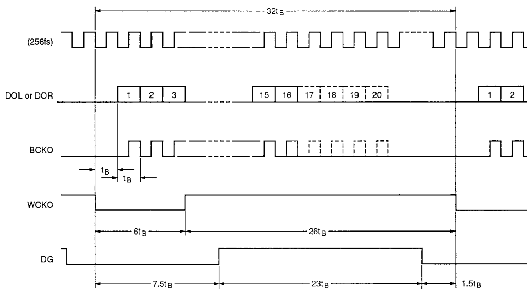
Figure 8. 8fs data output timing (OMOD = LOW, \overline{\text{CKSL}} = \text{LOW} )
