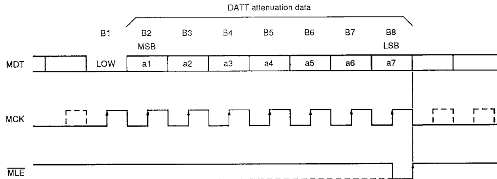
Figure 1. Attenuation data
