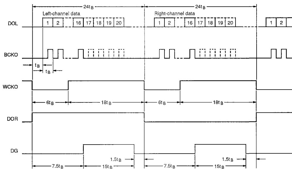
Figure 9. 4fs data output timing (OMOD = HIGH, \overline{\text{CKSL}} = \text{HIGH} )
