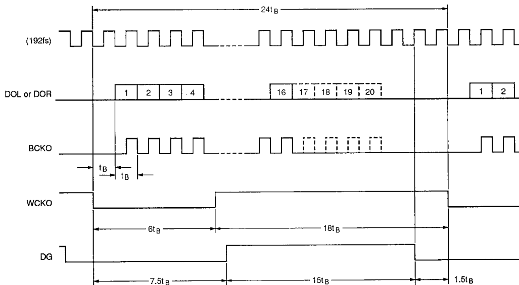
Figure 7. 8fs data output timing (OMOD = LOW, \overline{\text{CKSL}} = \text{HIGH} )
